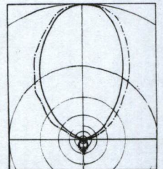
Model C.L.15 (20m) (21.3dBd) C.L.15 (15m) (28.7dBd) Model C.L.20 (20m) (14.2dBd)
